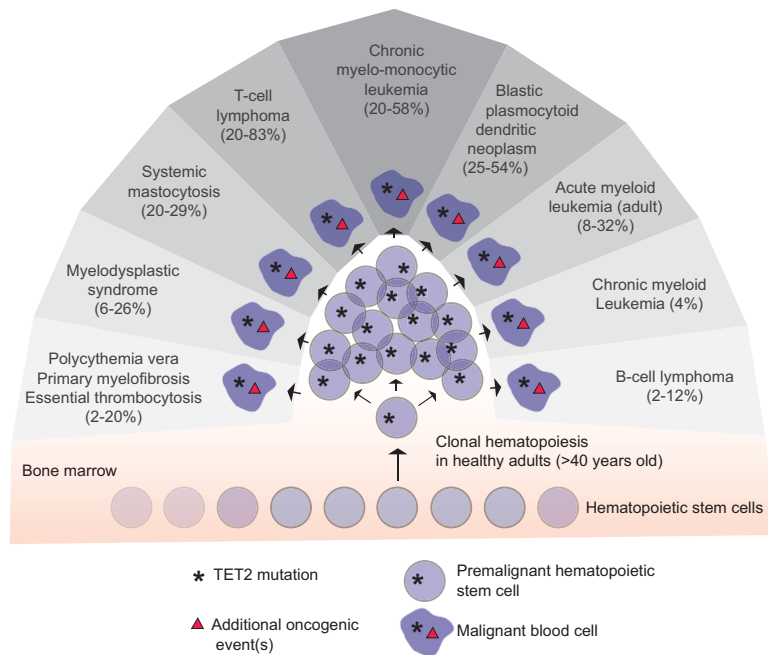
Figure 4. Illustration of the mutational landscape of TET2 in hematopoietic diseases. A somatic mutation in TET2 results in premalignant hematopoiesis and clonal expansion. Additional oncogenic events cooperate with the initial TET2 mutation to drive the onset of a wide variety of hematopoietic malignancies. The frequencies of TET2 mutations in the different patient groups are indicated (for review, see Scourzic et al. 2015).
